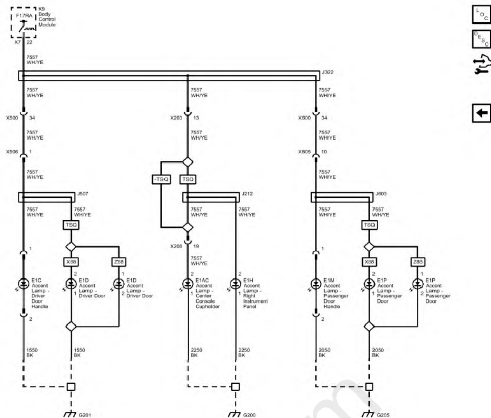
Fig. 20: Accent and Flood Lamps Courtesy of GENERAL MOTORS COMPANY
