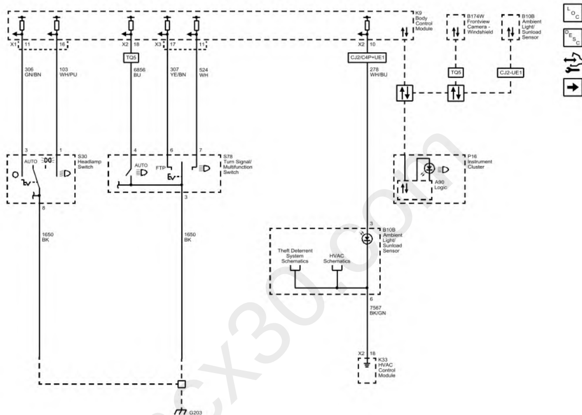
Fig. 1: Controls and Indicators
