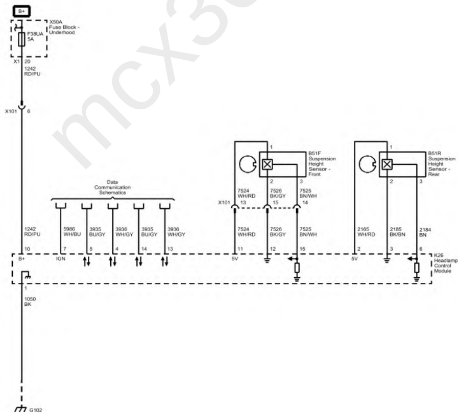
Fig. 7: Adaptive Forward Lighting - Power, Ground, Serial Data and Suspension Sensors (TR7) Courtesy of GENERAL MOTORS COMPANY
