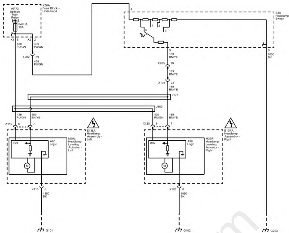
Fig. 6: Manual Headlamp Leveling (TR6) Courtesy of GENERAL MOTORS COMPANY
