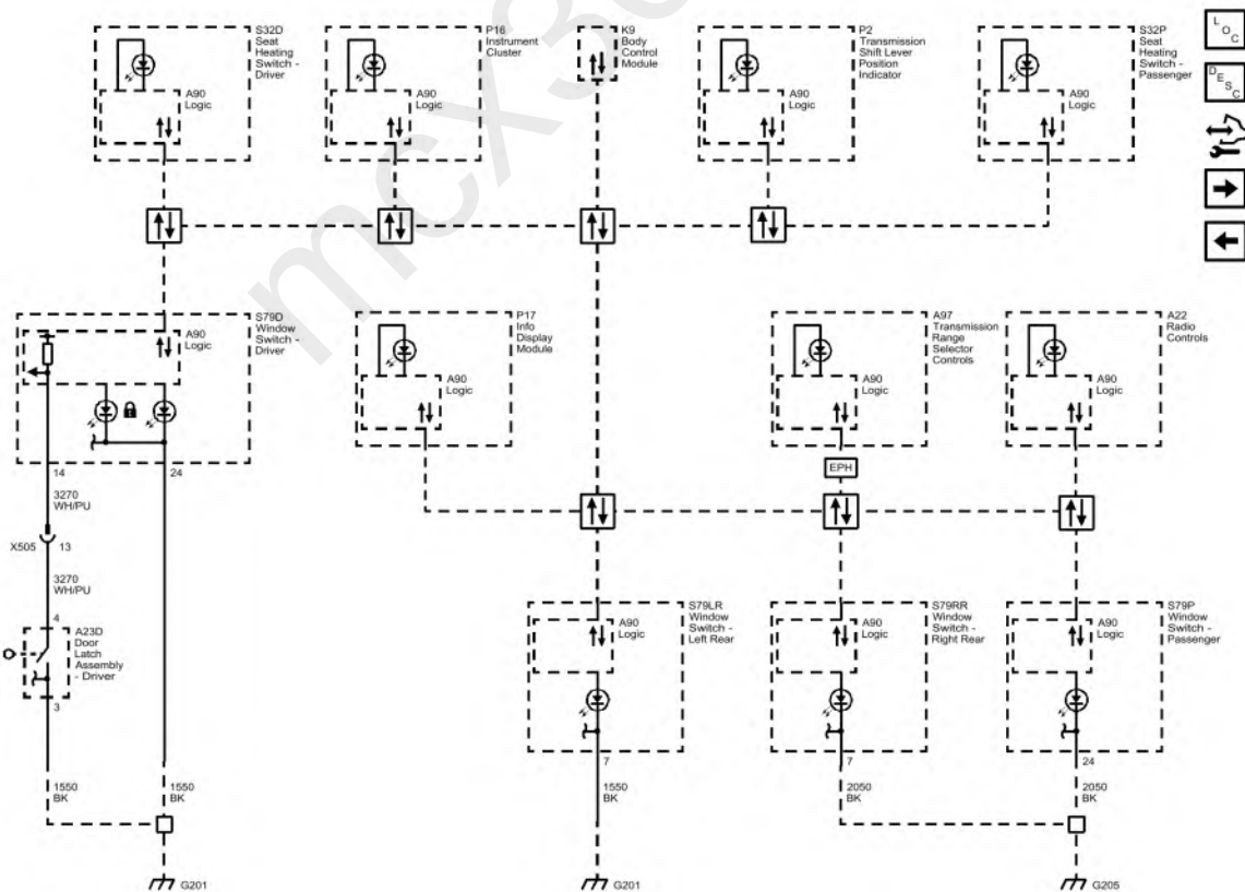
Fig. 23: Instrument Panel, Floor Console and Door Lamps - Serial Data Courtesy of GENERAL MOTORS COMPANY
