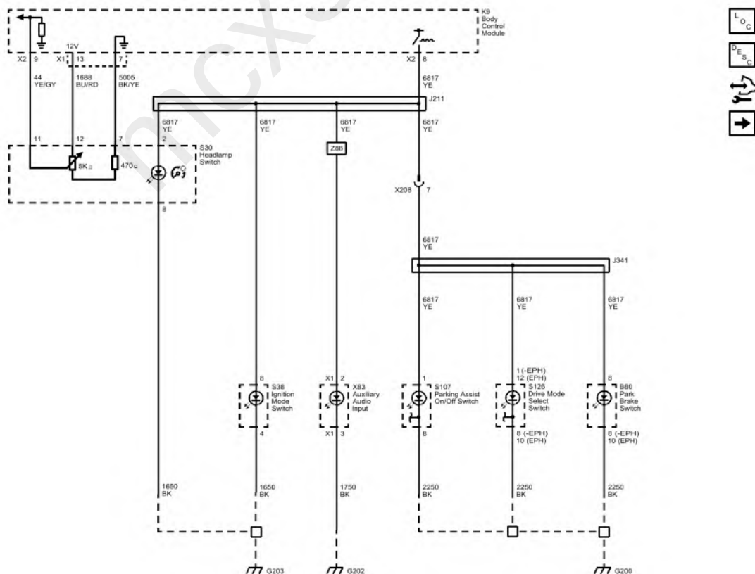
Fig. 21: Controls, Instrument Panel and Floor Console Lamps Courtesy of GENERAL MOTORS COMPANY
