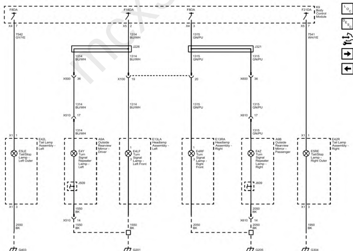
Fig. 11: Turn Signals (X88 without UGE) Courtesy of GENERAL MOTORS COMPANY
