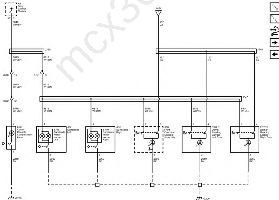
Fig. 19: Instrument Panel Compartment and Overhead Lamps Courtesy of GENERAL MOTORS COMPANY
