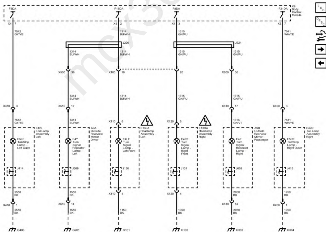
Fig. 13: Turn Signals (Z88) Courtesy of GENERAL MOTORS COMPANY
