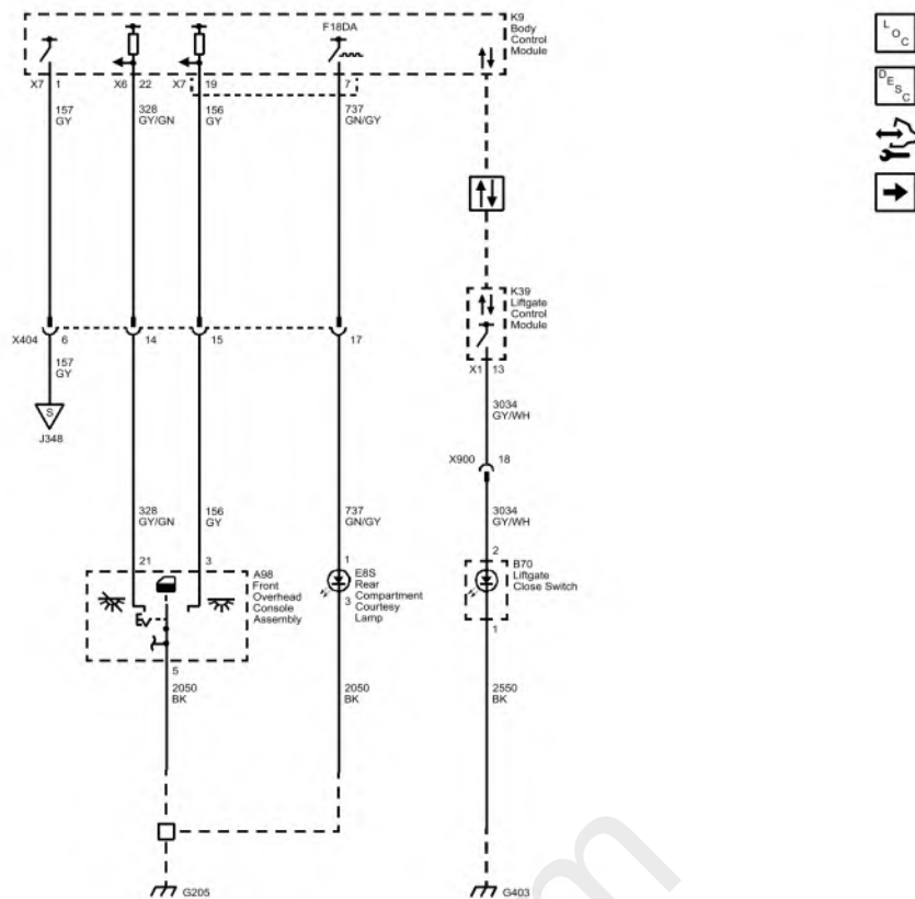
Fig. 18: Controls and Courtesy Lamps Courtesy of GENERAL MOTORS COMPANY
